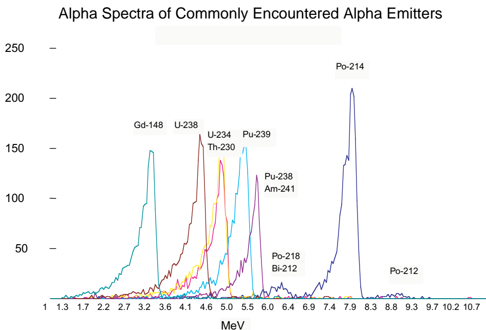
Figure 1. Alpha Spectra.
