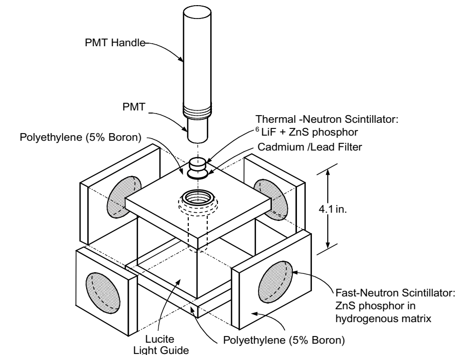
Figure 1. An exploded view of the PRESCILA neutron rem meter (patent pending).
