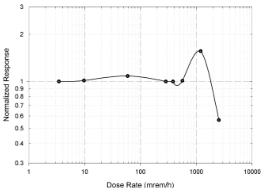
Figure 10. PRESCILA: response linearity.
